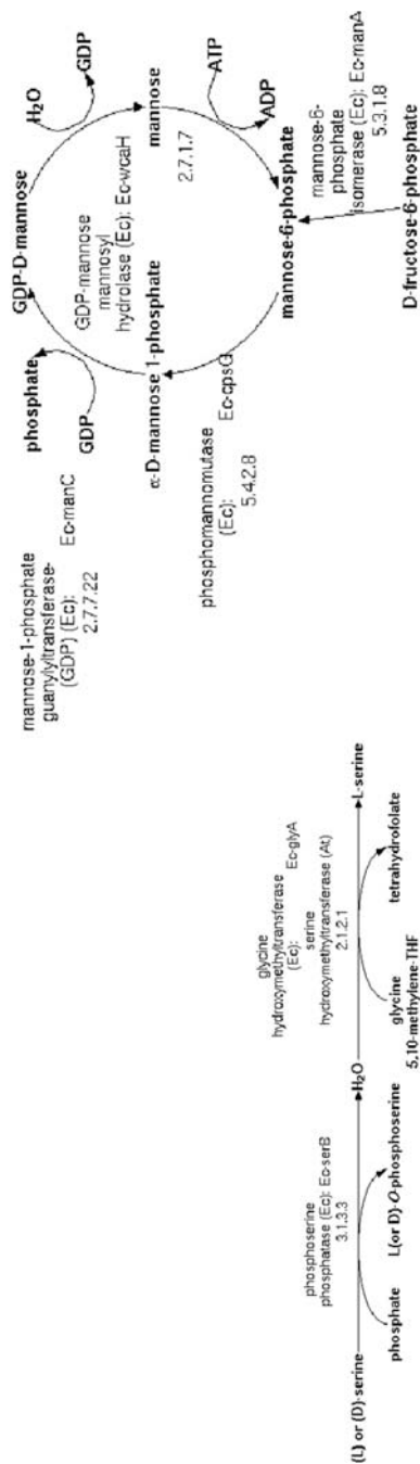
Fig. 17.1. Left: Glycine biosynthesis pathway. Right: GDP-mannose metabolism. (Pathway layouts were retrieved from the MetaCyc database (2)). Metabolic pathways are sequences of consecutive enzymatic reactions. Each reaction starts with a certain metabolite and produces another metabolite through synthesis, break down, or other transformations. The Glycine biosynthesis pathway produces the amino acid glycine from the amino acid serine. The GDP-mannose metabolism is one of the pathways that produce the compounds necessary to build cellular structures and organelles, such as cell walls.
